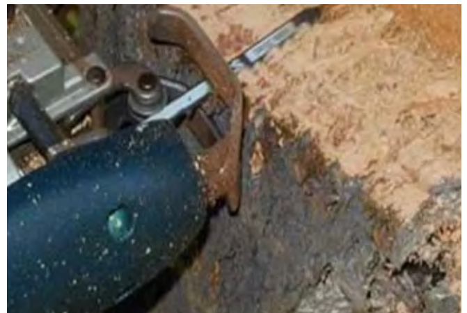
Figure 15: The cork debarking machine tested in Sardinia includes sensors capable of guiding it by measuring the different hydration of phellogen and cork (© The publication "The cultivation of cork oak").
